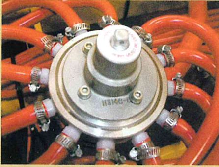
CDS - John Blue Flow Divider • Model FD1200 (12 outlet) • Model FD2000 (20 outlet)
